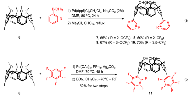
Scheme 3. Preparation of Fluorinated Calix[4]arenes 7–11
